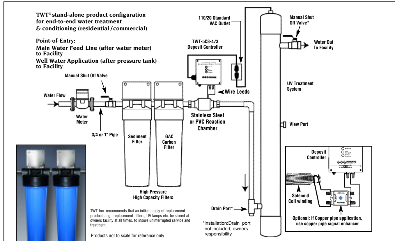
TWT-SYS700-FS-3/4" pipe size TWT-SYS1200-FS-1" pipe size Filter Set Systems Specs: Filter Housings 20" sediment filter 20" carbon filter Mounting Bracket Filter Wrench Pressure Tested
